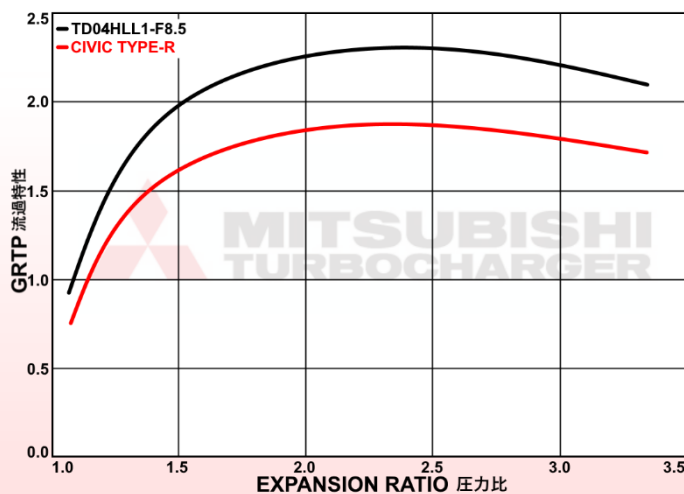
TURBINE MAP
