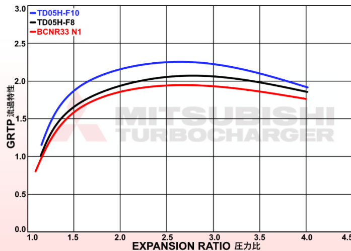
TURBINE MAP
