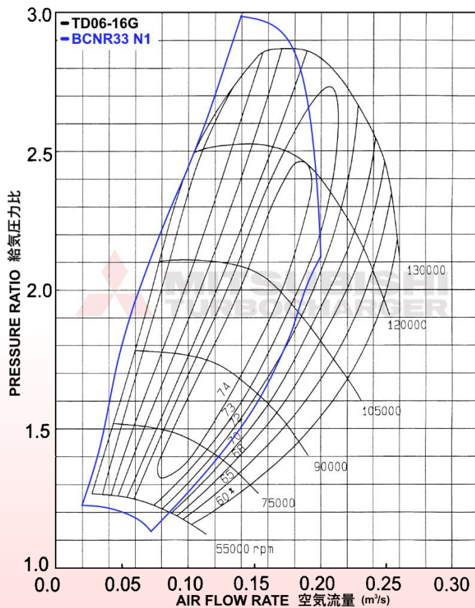
COMPRESSOR MAP
